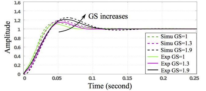
Fig. 13. Step responses with different gain scales. The overshoot in the experimental results, when GS is increased, matches our simulation predictions. The parameters are T_{qs} = T_{qd} = T_r = 1 ms, f_{qd} = 50 Hz, f_{rd} = 100 Hz, and f_n = 14 Hz.
