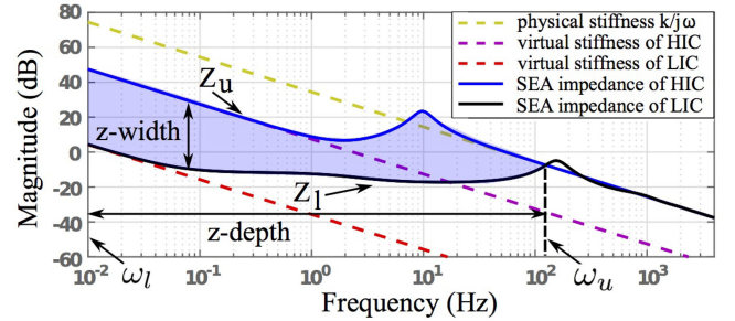
Fig. 10. Z-region surrounded by the highest impedance controller (HIC) and the lowest impedance controller (LIC). This figure shows achievable SEA impedance ranges by modulating the gain scale GS, as defined in Definition 1. The control gains are solved using the critically damped gain design criterion.
